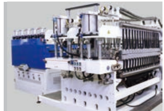
T-Die Head & Vacuum Calibration Unit
