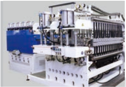
T-Die Head & Vacuum Calibration Unit
